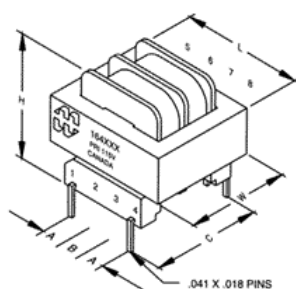
Single Primary 164 Series
