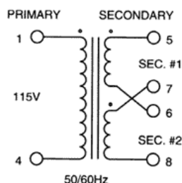
Single Primary 164 Series
