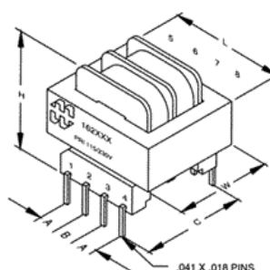
Dual Primary 162 Series
