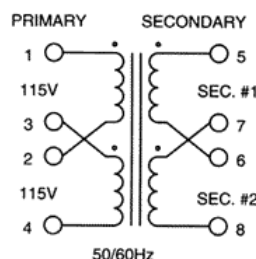
Dual Primary 162 Series
